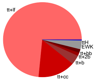
\geq 4 jets, 2 b-tags
