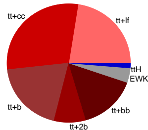
\geq 4 jets, 3 b-tags
