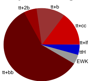
\geq 4 jets, \geq 4 b-tags
