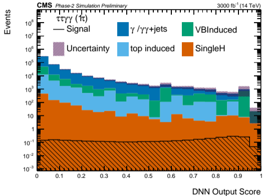
(b) One tau final state
