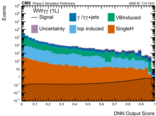
(a) One Lepton final state
