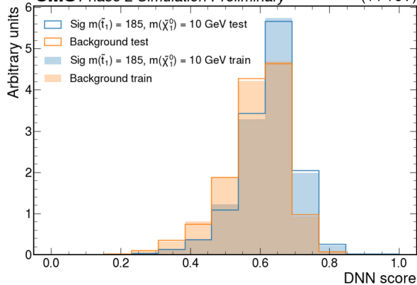
CMS Phase 2 Simulation Preliminary (14 TeV)
