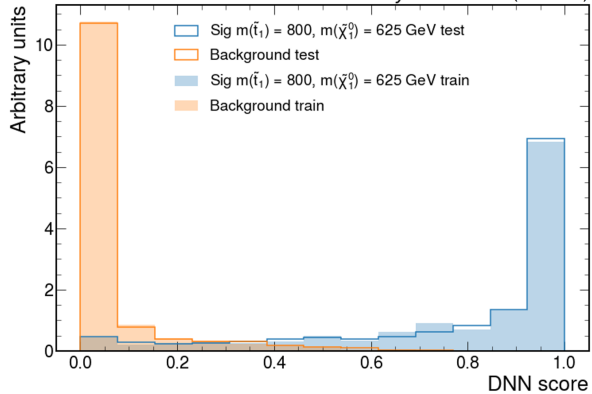
CMS Phase 2 Simulation Preliminary (14 TeV)
