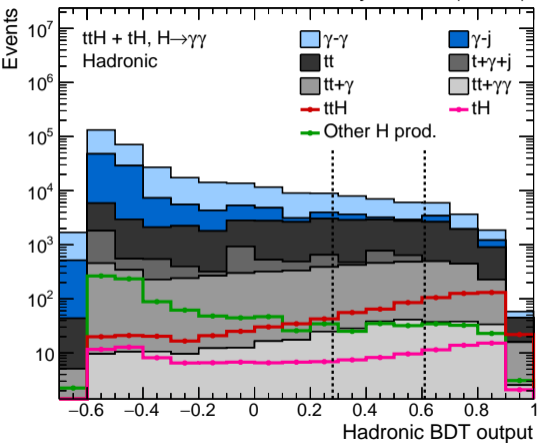
CMS Phase-2 Simulation Preliminary 3 \text{ ab}^{-1} (14 TeV)
