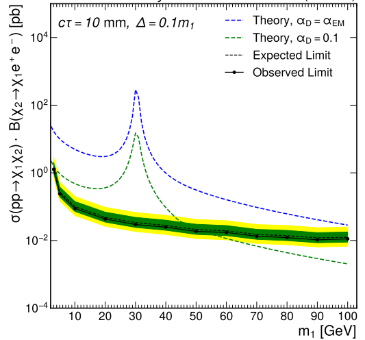
CMS Preliminary 138 fb -1 (13 TeV)
