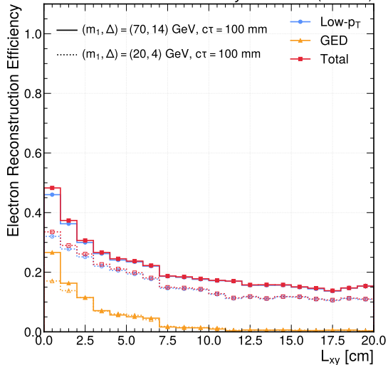
CMS Simulation Preliminary 138 fb -1 (13 TeV)
