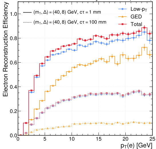
CMS Simulation Preliminary 138 fb -1 (13 TeV)
