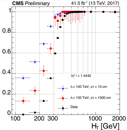
L1T+HLT efficiency
