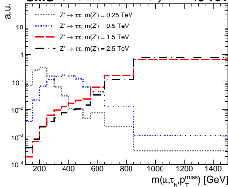
CMS Simulation Preliminary 13 TeV
