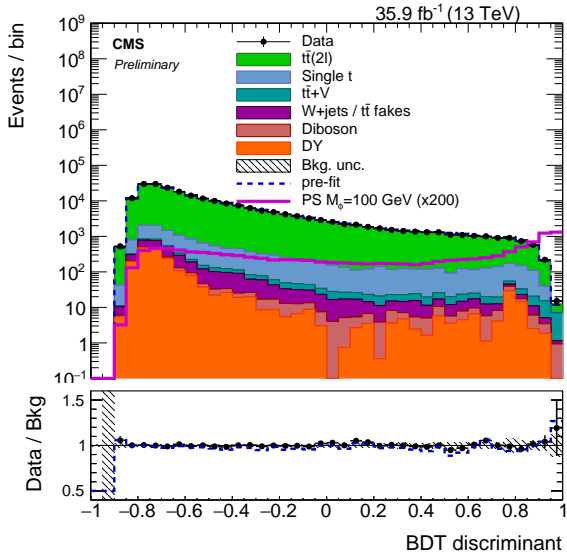
(b) pseudoscalar training
