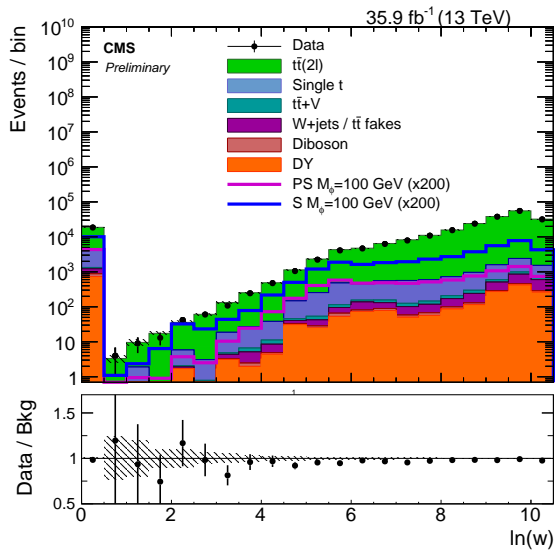
(b) log of kinematic reconstruction weight \ln w
