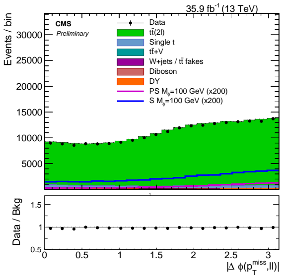
(a) |\Delta\phi(p_T^{\text{miss}}, ll)|
