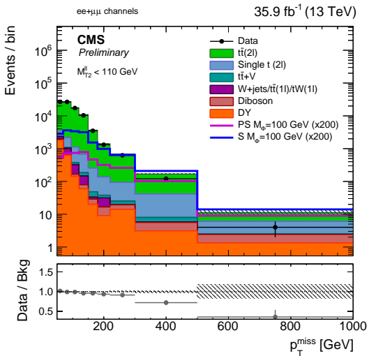
(b) low purity, ee + \mu\mu channels
