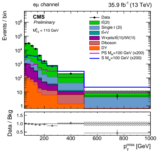
(a) low purity, e\mu channel
