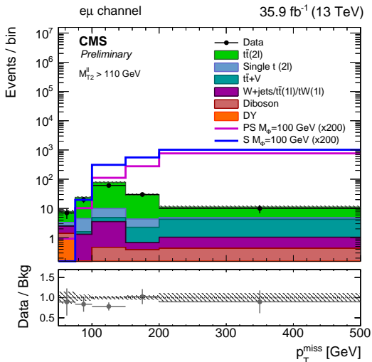
(c) high purity, e\mu channel
