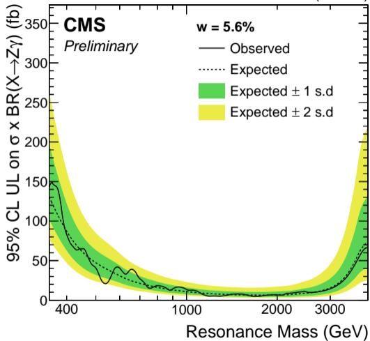
(b) \frac{\Gamma}{m} = 5.6\% : combination
