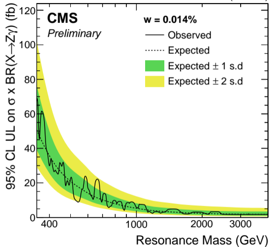
(a) \frac{\Gamma}{m} = 0.014\% : combination
