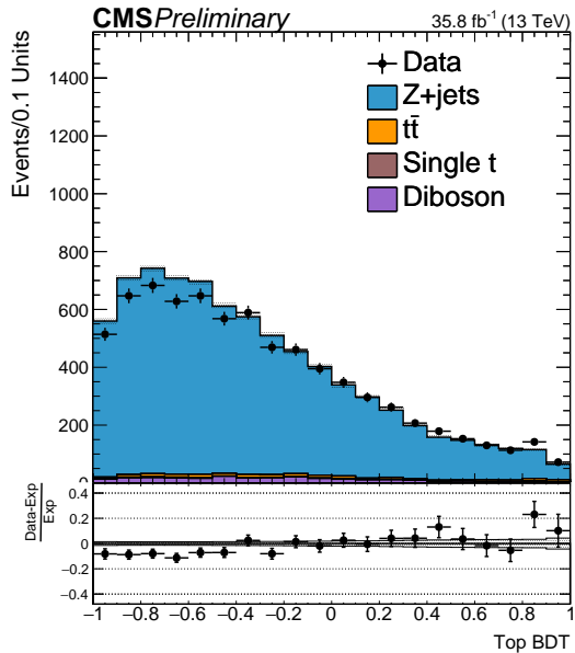
(b) Z \rightarrow \mu\mu selection
