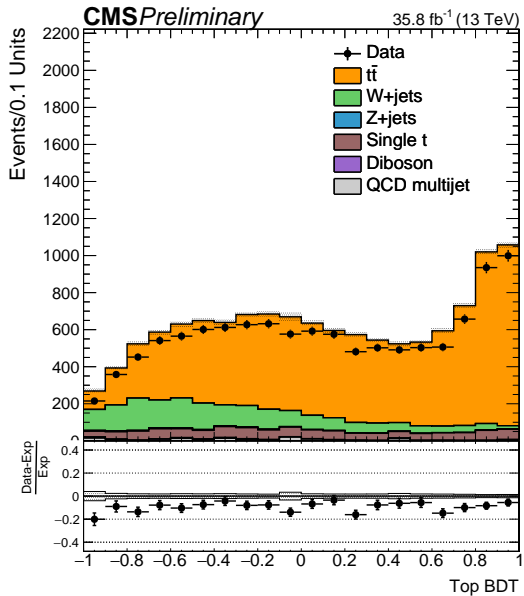
(a) Single muon t\bar{t} selection
