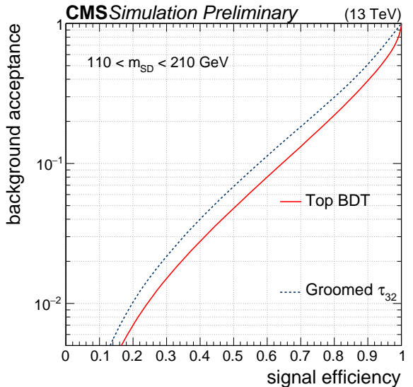
(b) Comparison of performance of the BDT and \tau_3/\tau_2
