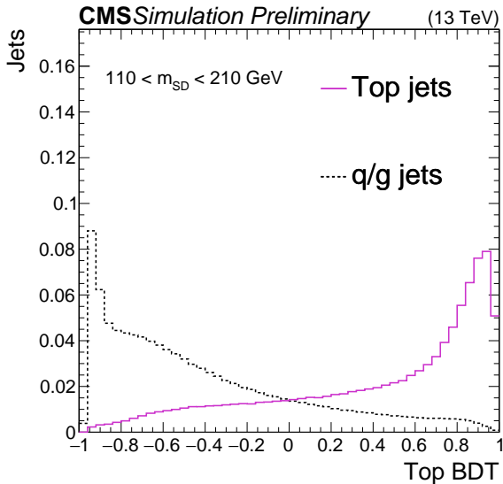
(a) BDT response in top and q/g jets
