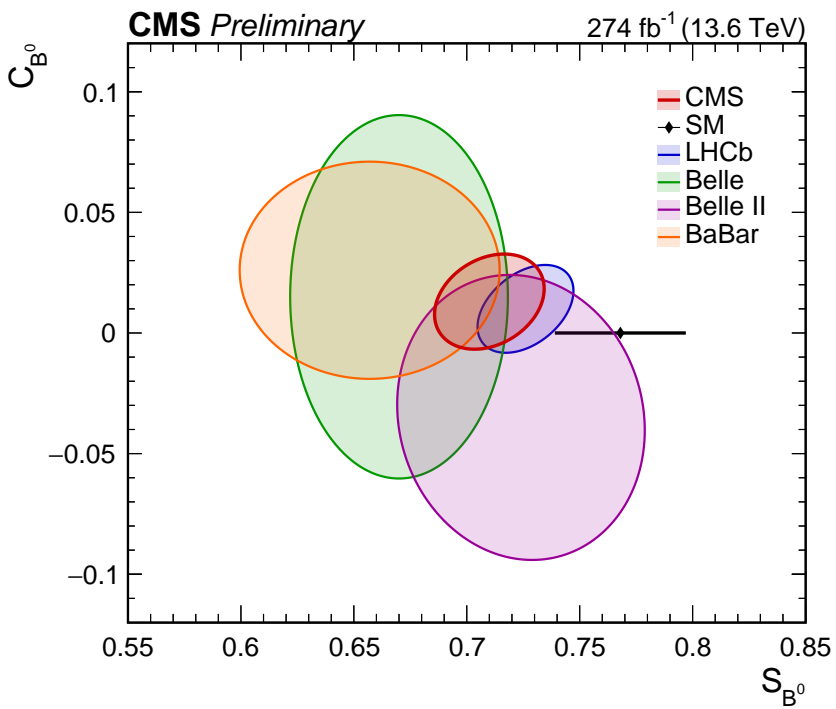
(a) B^0 \rightarrow J/\psi K_S^0 measurement.
