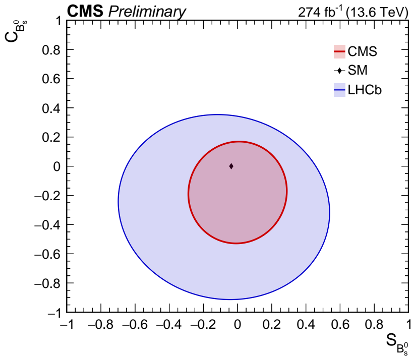
(b) B_s^0 \rightarrow J/\psi K_S^0 measurement.
