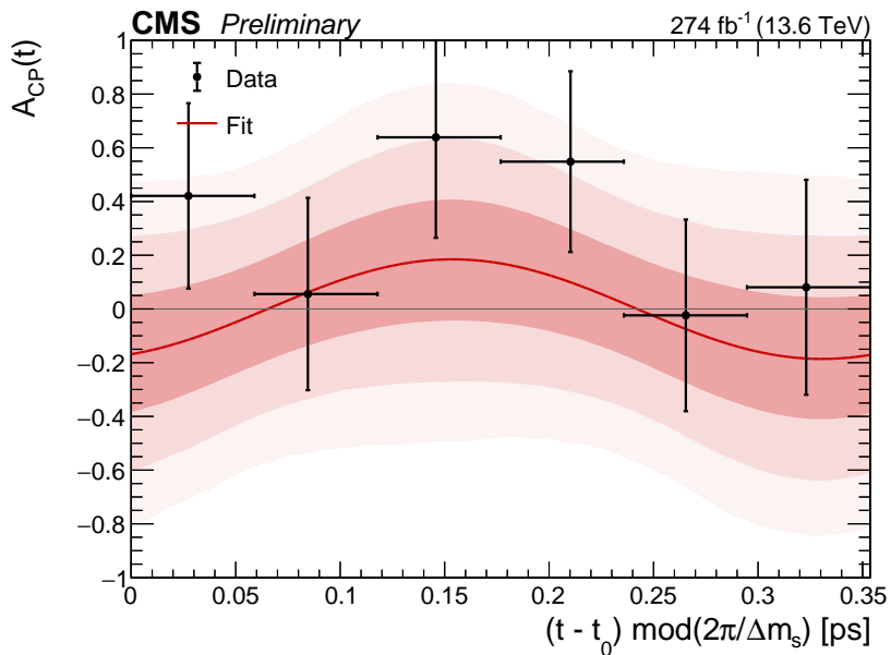
(b) B_s^0 \rightarrow J/\psi K_S^0 decay channel.
