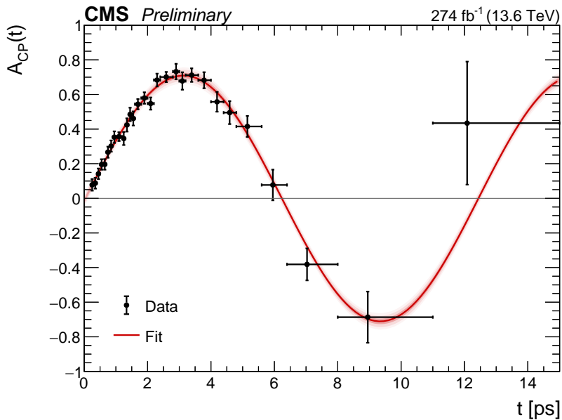
(a) B^0 \rightarrow J/\psi K_S^0 decay channel.
