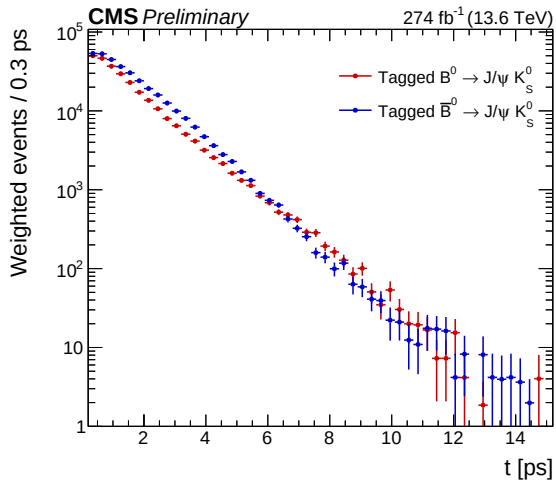
(a) B^0 \rightarrow J/\psi K_S^0 COW-weighted decays.
