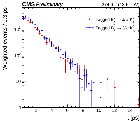
(b) B_s^0 \rightarrow J/\psi K_S^0 COW-weighted decays.
