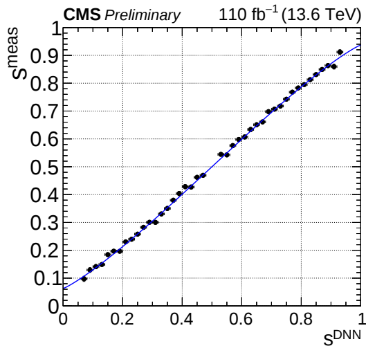
(b) OS-electron tagger.
