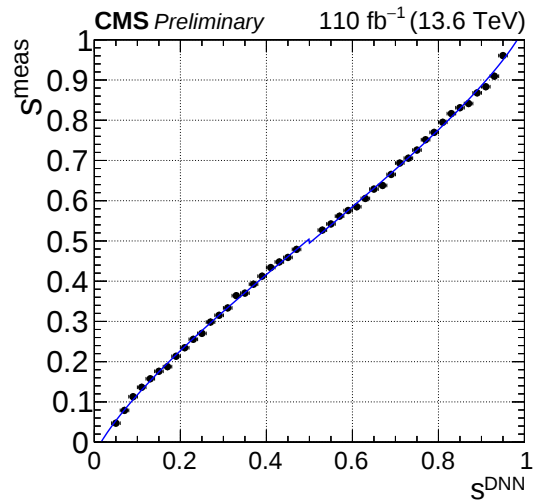
(a) OS-muon tagger.
