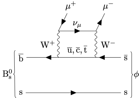
(b) Box diagram
