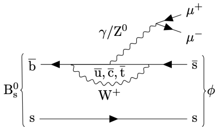
(a) Penguin diagram
