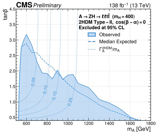
(a) ( m_A, \tan\beta ) for m_H = 400 GeV
