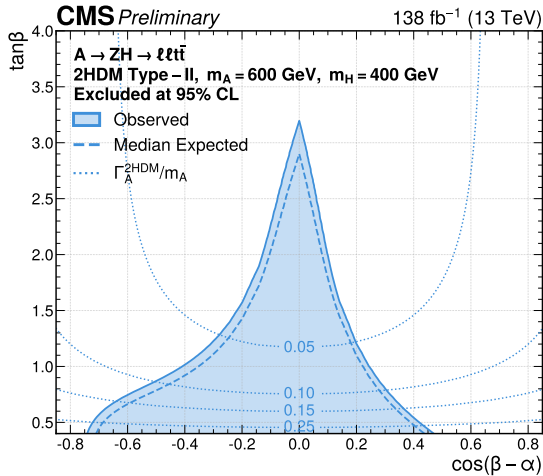
(b) ( \cos(\beta - \alpha), \tan\beta ) for (m_A, m_H) = (600, 400) GeV
