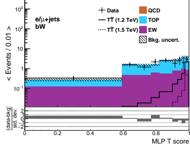
CMS Preliminary 137 fb -1 (13 TeV)
