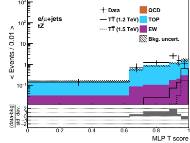
CMS Preliminary 137 fb -1 (13 TeV)
